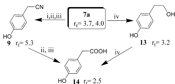
Scheme 4. Metabolism of 4-hydroxyphenylacetaldoxime ( 7a ) by fungi: (i) Phoma lingam BJ-125; (ii) Sclerotinia sclerotiorum clone #33; (iii) Rhizoctonia solani AG 2-1; (iv) Beauveria bassiana ATCC 7159; R_t = HPLC retention time in min using mobile phase A (see Experimental).
