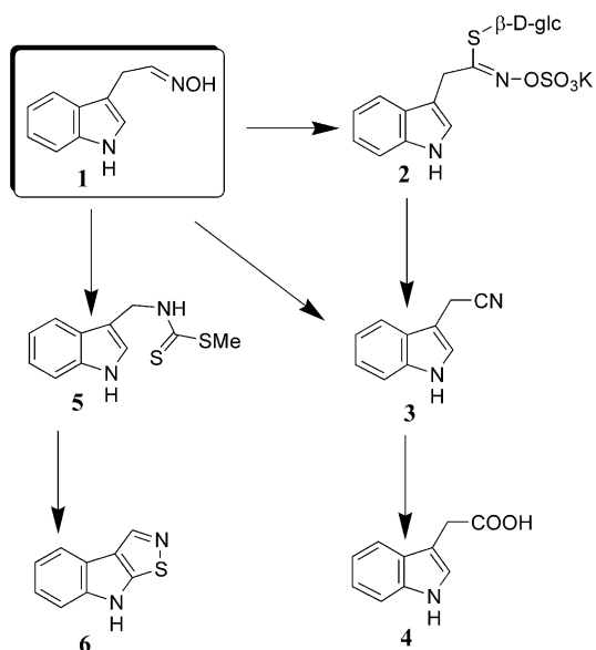
Scheme 1. Metabolism of indole-3-acetaldoxime ( 1 ) in cruciferous plants. 1–5
