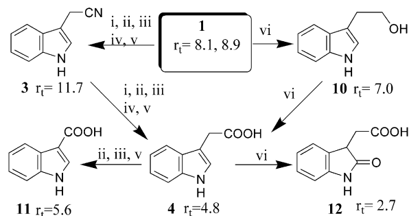
Scheme 3. Metabolism of indole-3-acetaldoxime ( 1 ) by fungi: (i) Phoma lingam BJ-125; (ii) P. lingam Laird 2; (iii) P. lingam Mayfair 2; (iv) Sclerotinia sclerotiorum clone #33; (v) Rhizoctonia solani AG 2-1; (vi) Beauveria bassiana ATCC 7159; R_t = HPLC retention time in min using mobile phase A (see Experimental).
