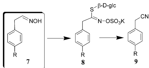
Scheme 2. Metabolism of 4-substituted-phenylacetaldoxime ( 7 ) in cruciferous plants. 3,4
